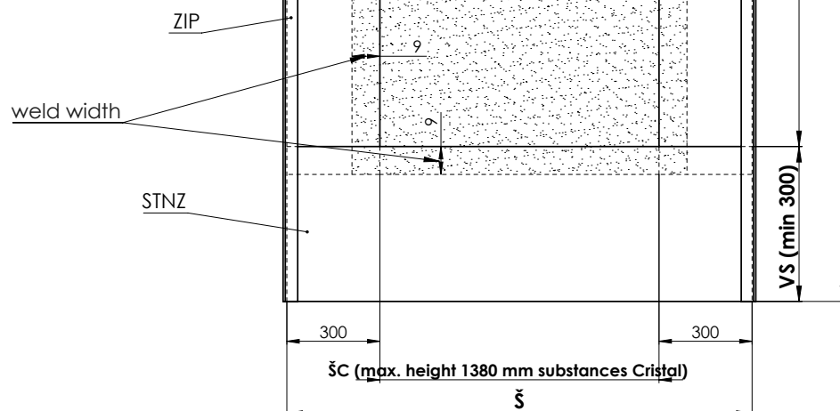
OPTION OF THE VERTICAL FABRIC CRISTAL FOR PRODUCTS SCREEN ZIP AND SCREEN ZIP ECONOMY
