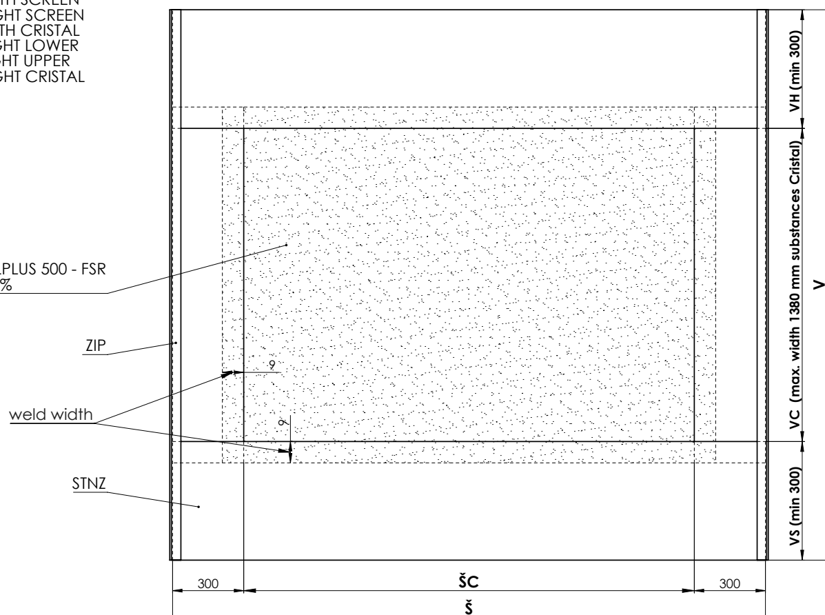
OPTION OF THE HORIZONTAL FABRIC CRISTAL FOR PRODUCT SCREEN ZIP AND SCREEN ZIP ECONOMY
