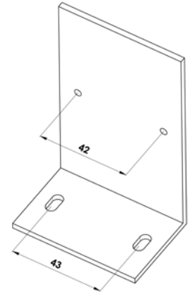
Square L (7-302233)
