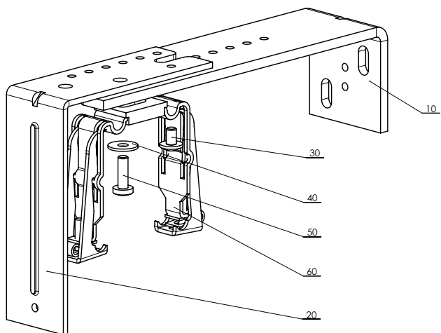
Adjustable bracket - mechanical 206 – 268 mm P 010/36 (2-01794-0000)
