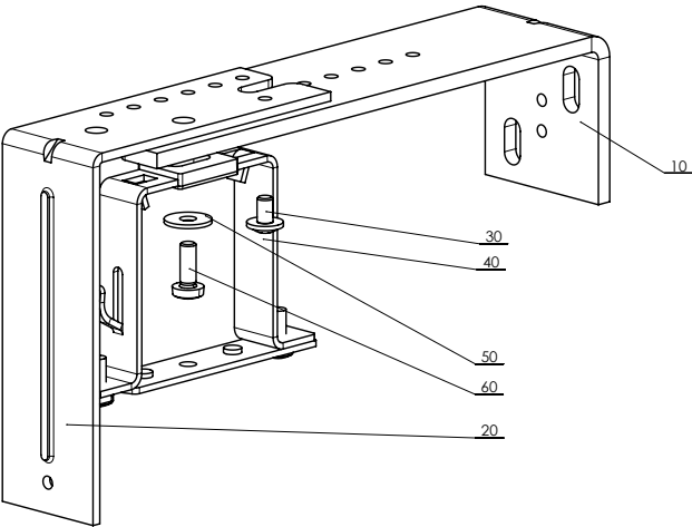
Adjustable bracket – fixed 206 – 268 mm P 010/42 (2-01800-0000)
