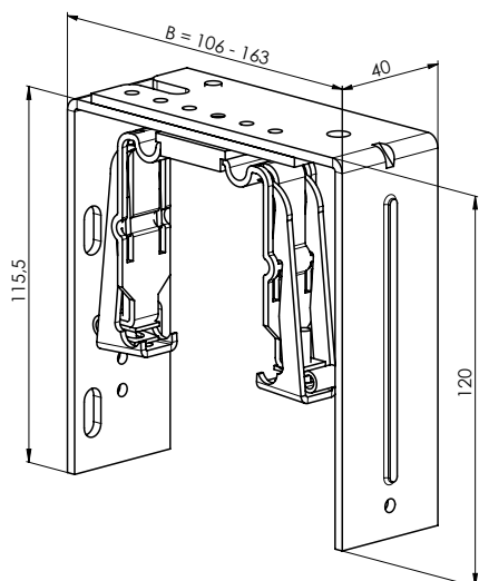
Blind bracket - short, adjustable and mechanical 106-163 mm P 009/21 (2-01392) (for head rail 56 x 58)
