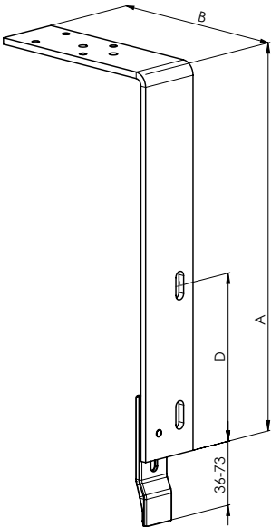
Variable holder P 130/4 2-01419-0000-0
