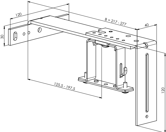
Adjustable hanger - fixed 217 - 277 mm P 010/35 (2-01604-0000)
